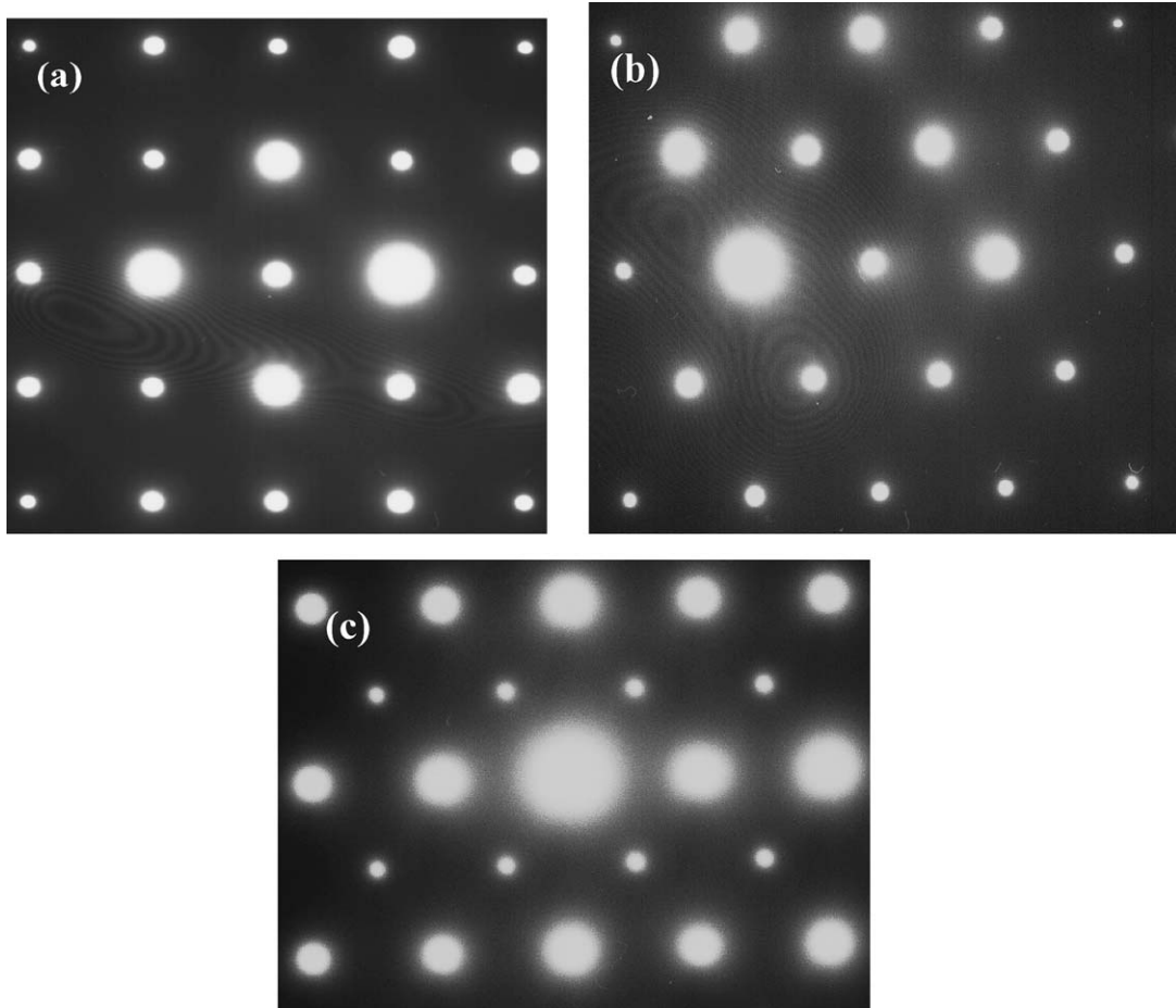
Fig. 2. Electron diffraction patterns along (a) \langle 100 \rangle , (b) \langle 111 \rangle and (c) \langle 110 \rangle .
